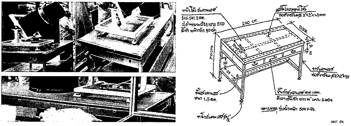
Figure 9: Example of table for holding satellite*
